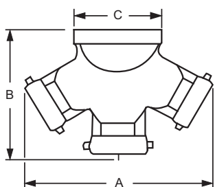
back outlet connection 21-205
