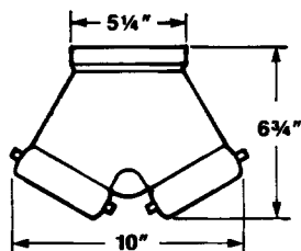
Fig. 5710 ... Back Outlet U/L Listed FM Approved
