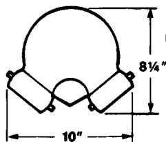
Fig. 5715 ... Angle Outlet U/L Listed FM Approved
