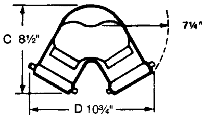
Fig. 5730 Series 90° Angle Outlet
