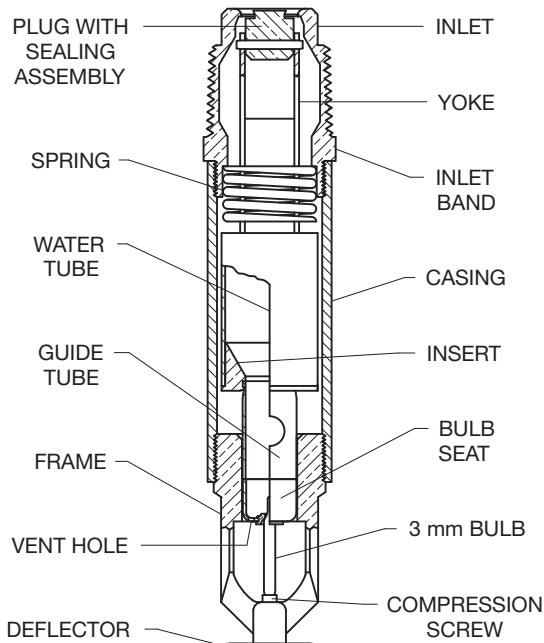
FIGURE 2 SERIES DS-1, 1 INCH NPT AND ISO 7-R 1 DRY-TYPE SPRINKLER ASSEMBLY
