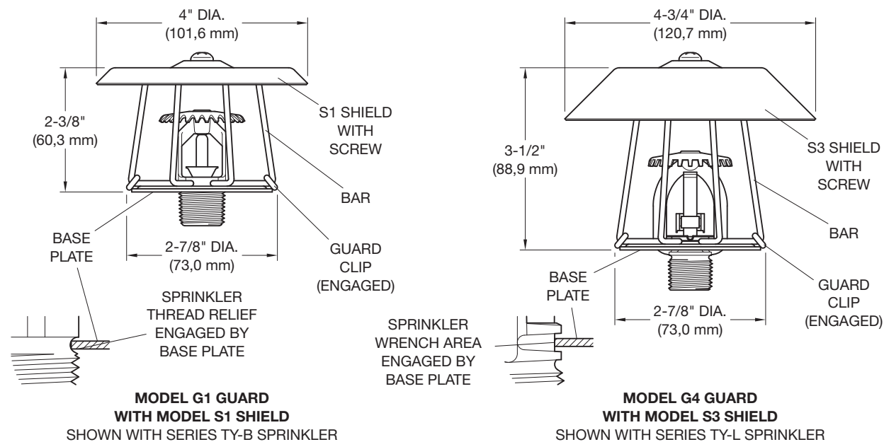
FIGURE 2 MODEL G1/S1 AND G4/S3 SPRINKLER GUARDS WITH SHIELDS — DIMENSIONS —
