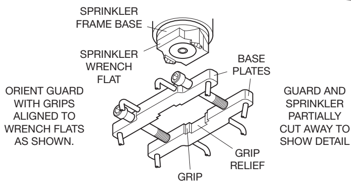
FIGURE 2B MODEL G5 SPRINKLER GUARD — INSTALLATION STEP 2 —
