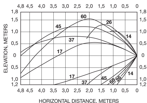
FIGURE 3 TYPE HV NOZZLES OVERALL VERTICAL SPRAY PATTERNS WHEN PROJECTING WATER HORIZONTALLY BEYOND THE DESIGN PARAMETERS IN FIGURE 2 30 to 80 PSI (2,1 to 5,5 bar)
