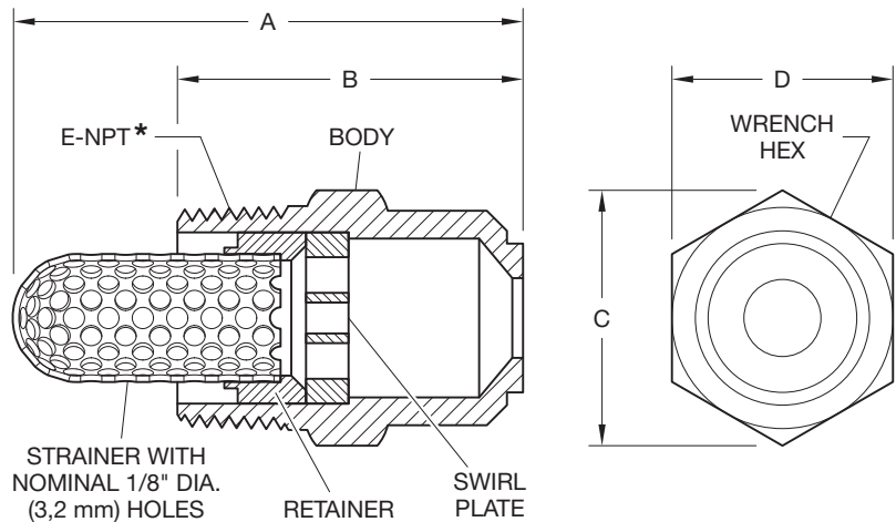
TYPE HV-37, HV-45, AND HV-60
