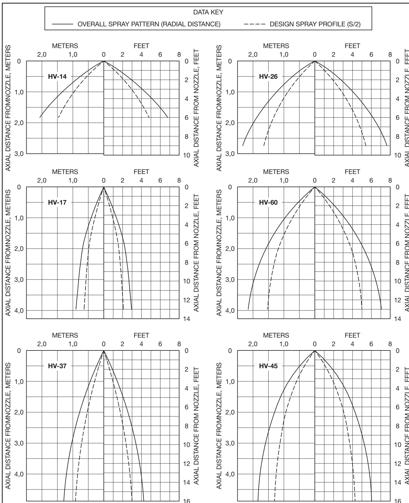
FIGURE 2 — PART 1 OF 2 TYPE HV NOZZLES WATER DISTRIBUTION DESIGN DATA
