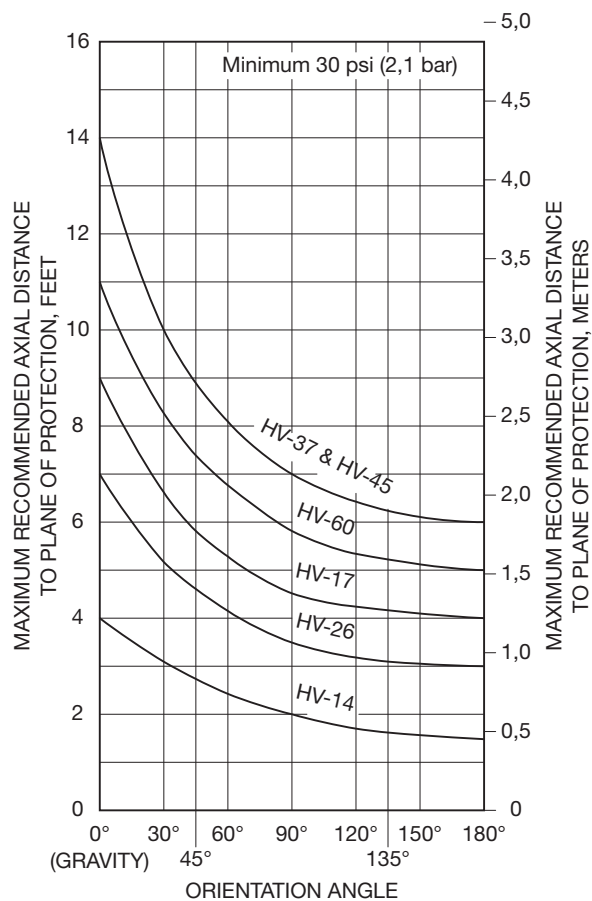
FIGURE 2 — PART 2 OF 2 TYPE HV NOZZLES WATER DISTRIBUTION DESIGN DATA
