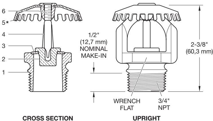
FIGURE 1 ULTRA K17, 155°F (68°C) & 200°F (93°C), UPRIGHT SPRINKLER (TY7153)
