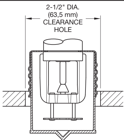
FIGURE 3 DISPOSABLE PROTECTIVE CAP
