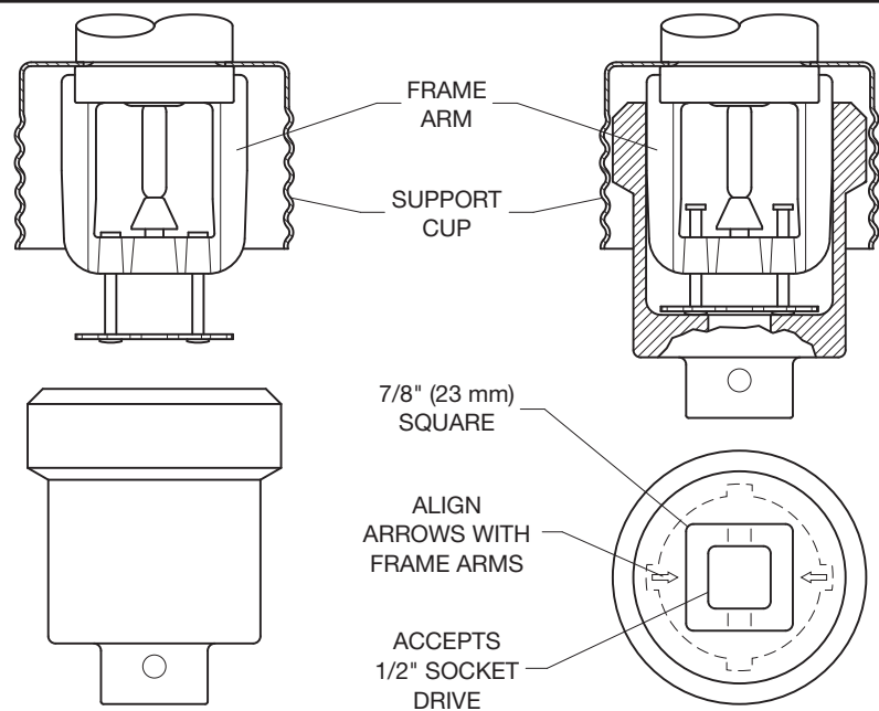
FIGURE 4 RFII SPRINKLER WRENCH
